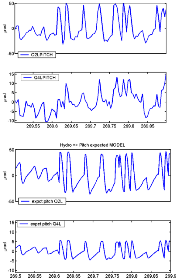
Figure 10: Measured (two top graphs) and modeled (two bottom graphs) signals from the left side tiltmeters corresponding to the reconstructed motion shown in Figure 8. Horizontal scale shows the day of 2003.
