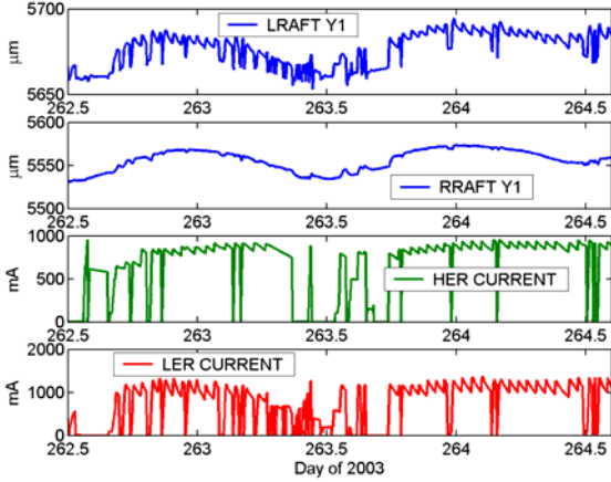
Figure 5: Raw signals from HLS sensors located most close to the IP on the left and right sides and the HER and LER beam currents.
