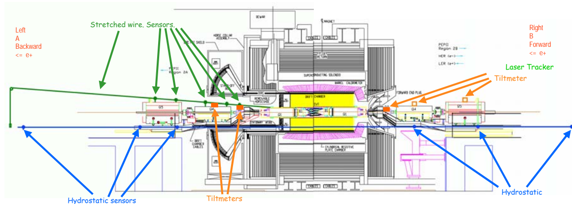
Figure 3: PEP-II IR scheme with hydrostatic system, stretched wire and tiltmeters (drawing courtesy Stuart Metcalfe).
