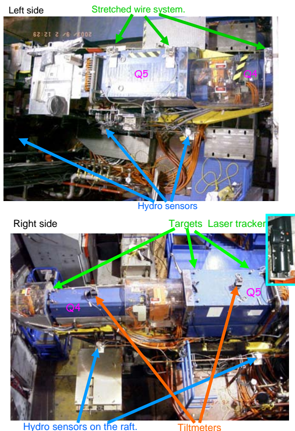
Figure 4: Photo of the left and right rafts supporting Q5, Q4 and Q2 magnets (part of Q2 is visible on the right side, under the plastic cover). Locations of hydrostatic sensors, stretched wire sensors (installed on the left side only), tiltmeters, laser tracker and its targets (installed on the right side only) are shown by arrows.
