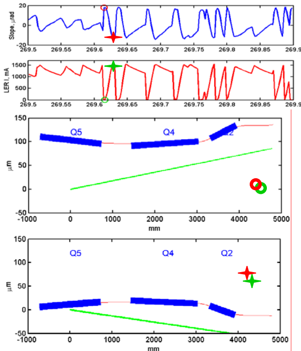
Figure 8: The left raft slope and LER current for the time interval used for magnet motion reconstruction, two top graphs (horizontal scale shows day of 2003). The bottom two graphs show reconstructed motion of the left side magnets for two extreme values of LER current. The green line indicates position of the raft and the blue boxes indicate positions of the Q5, Q4 and Q2 magnets (horizontal axis shows the distance along the beamline with respect to position of the central raft support).
