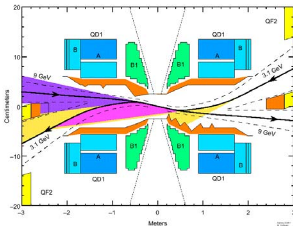
Figure 1: Schematics of PEP-II interaction region with synchrotron radiation fans from LER beam (picture courtesy Mike Sullivan).
