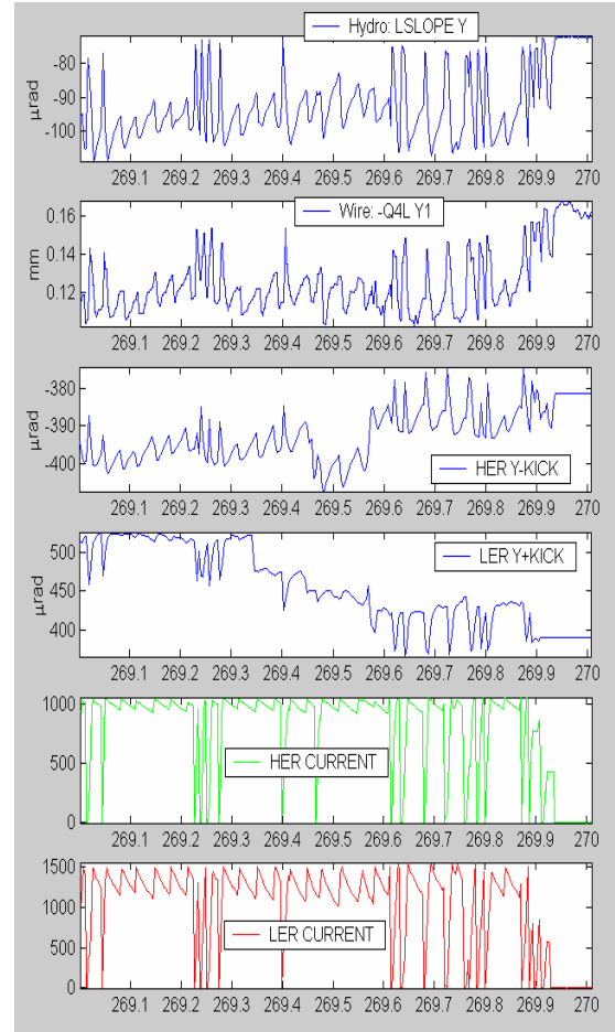
Figure 7: Slope of the left raft, signal of the stretched wire system, signals from the HER and LER orbit feedbacks, and beam currents. Horizontal axis shows the day of 2003.
