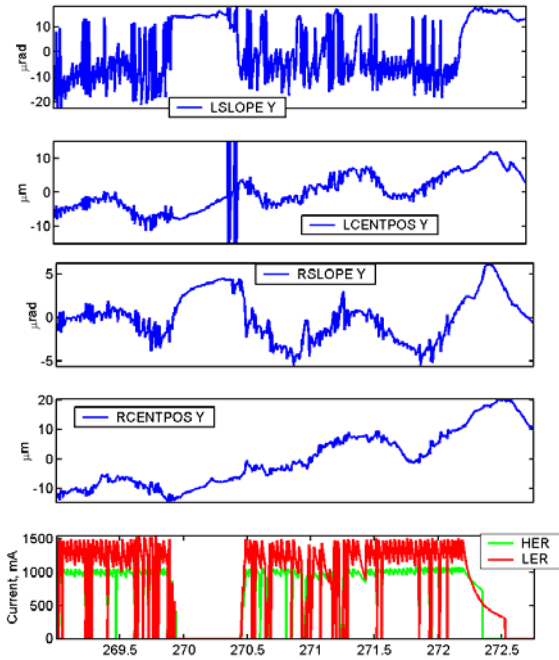
Figure 6: Data from HLS sensors converted into position of the raft central support point and its pitch. Horizontal axis shows the day of 2003.
