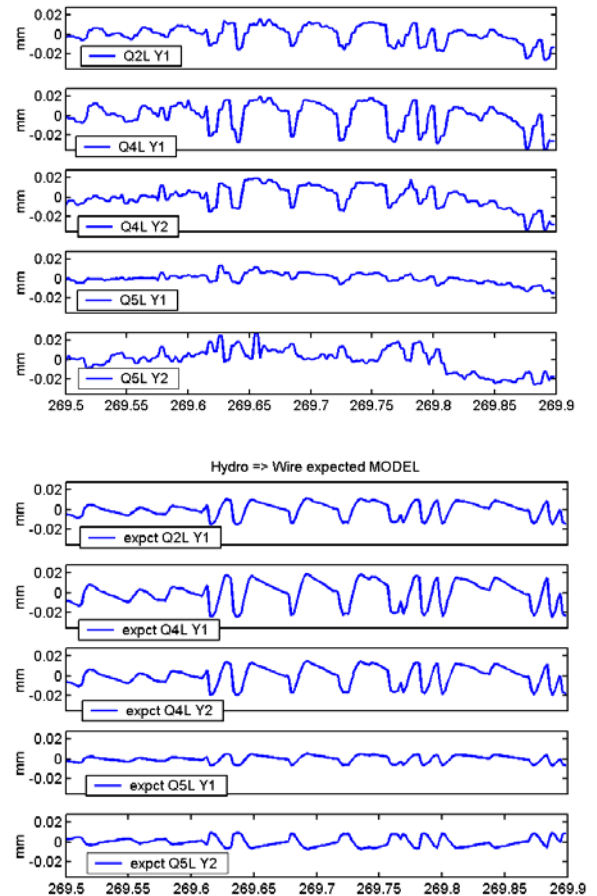
Figure 9: Measured (five top graphs) and modeled (five bottom graphs) signals of the stretched wire system corresponding to the reconstructed motion shown in Figure 8. Horizontal scale shows the day of 2003.
